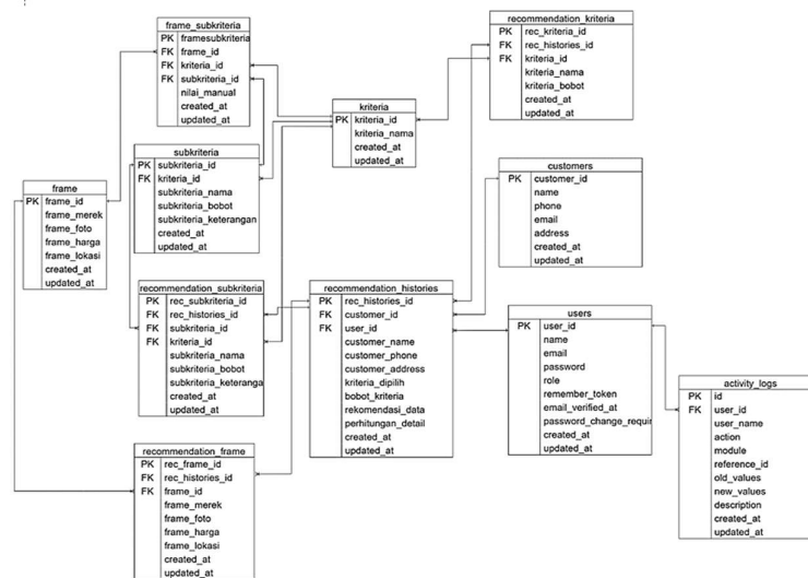
Gambar 8. Entity Relationship Diagram
