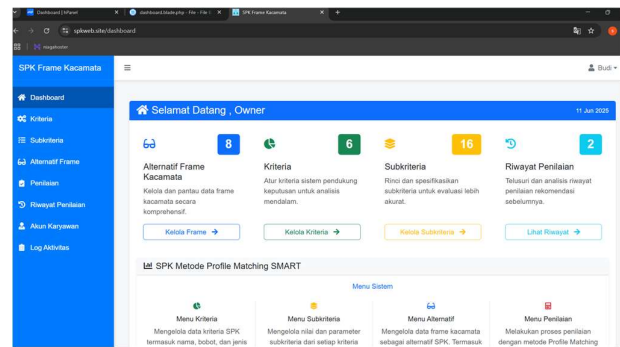
Gambar 11. Halaman Dashboard
