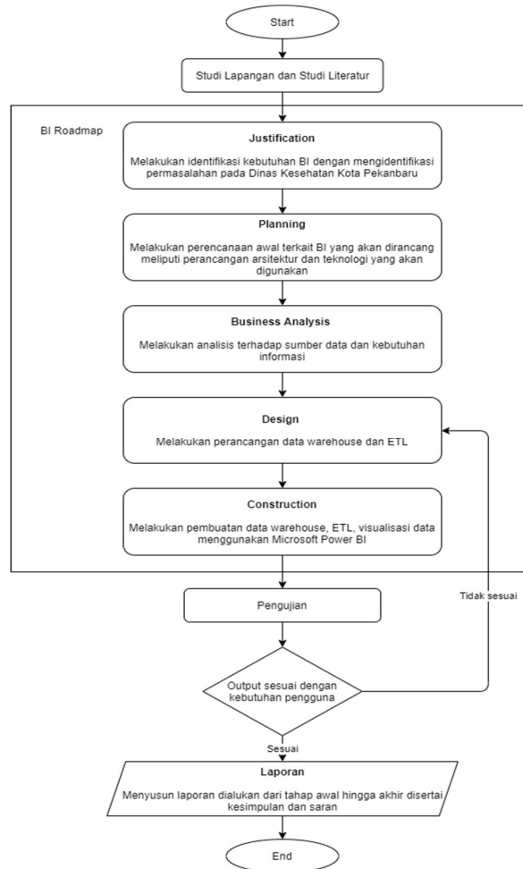
Gambar 1. Flowchart Penelitian
