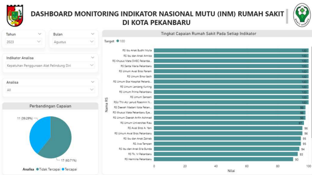
Gambar 1. Dashboard Monitoring
