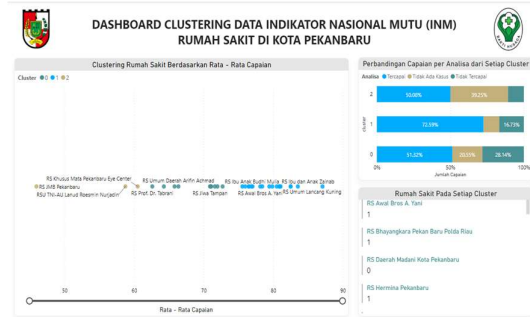
Gambar 11. Dashboard Clustering
